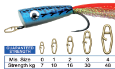
240163 - Stonfo 636 QUICKLINK ROUNDED MIS. 0-1-2-3-4
