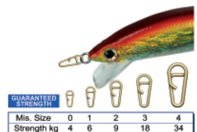
240163 - Stonfo 636 QUICKLINK ROUNDED MIS. 0-1-2-3-4
