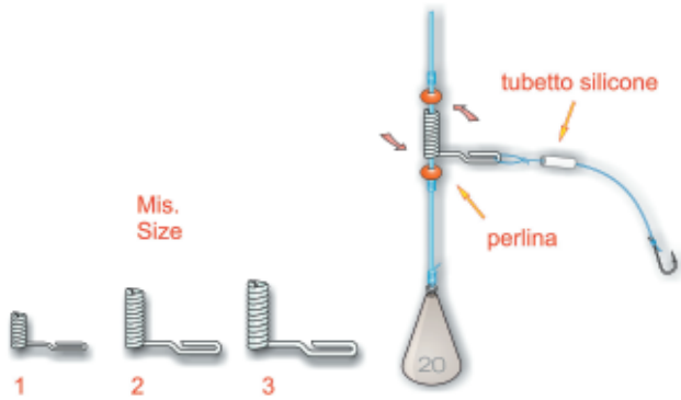
240032 - FAST CONNECTOR LIGHT - Art. 346
